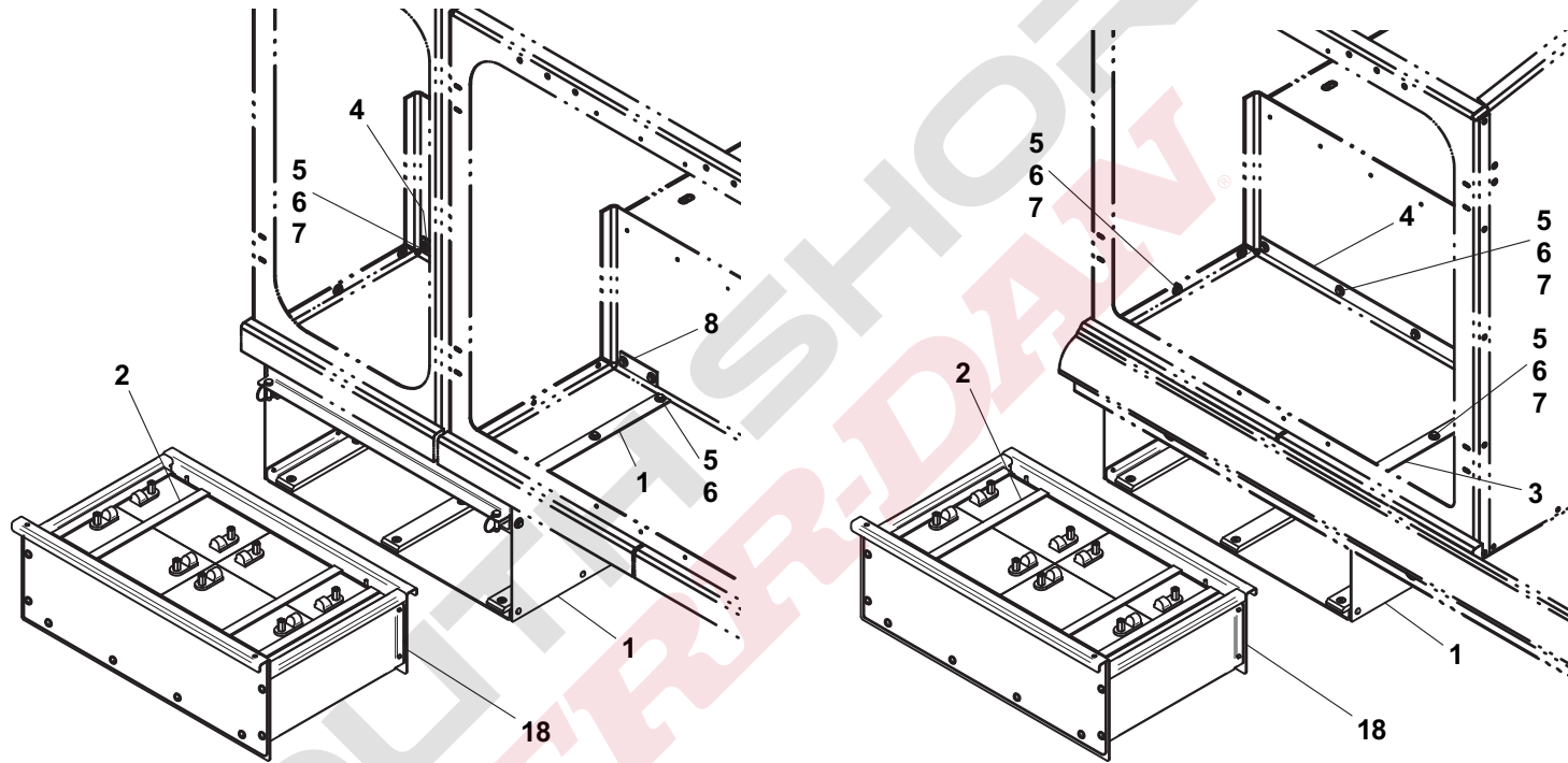
UNDER BODY BATTERY BOX MOUNTED AT 24" TUNNEL TOOLBOX
